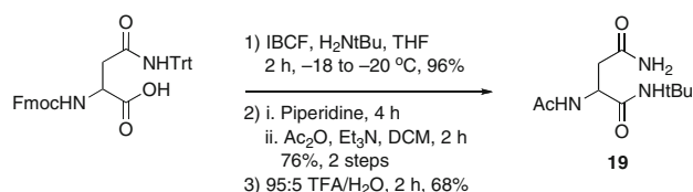
Scheme 7 Synthesis of Asn derivative substrate 19 via N -Fmoc and trityl protection
