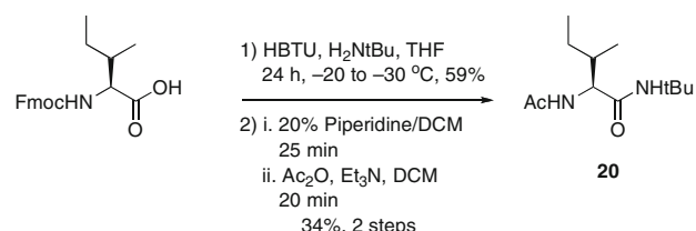
Scheme 8 Synthesis of Ac-Ile-NHtBu via N -Fmoc protection
