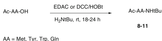
Scheme 3 Synthesis of substrates 8–11 via direct condensation; starting from N -acetyl amino acids
