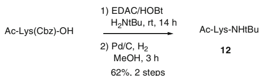
Scheme 4 Synthesis of 12 via direct condensation of N -acetyl-Lys(Cbz)-OH with tert -butylamine followed by hydrogenation of the CBz protecting group
