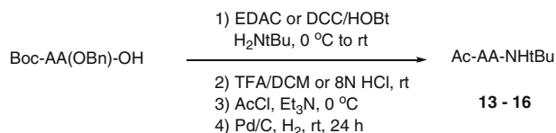
Scheme 5 Synthesis of substrates 13–16 via Boc-AA(OBn)-OH
